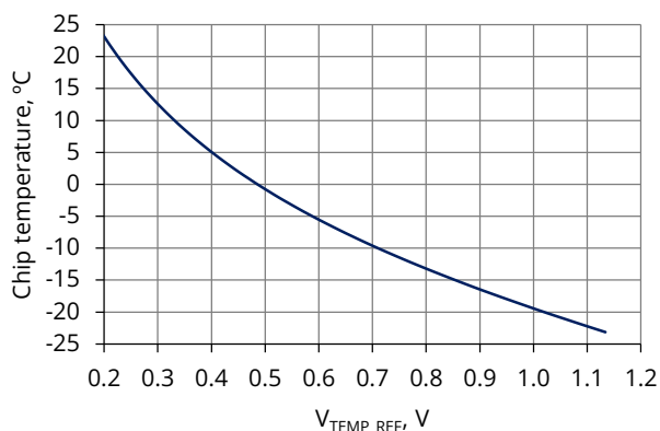
FIGURE 6. Detection chip temperature vs voltages on TEMP_REF and TEMP_OUT pins (see FIGURE 12)
