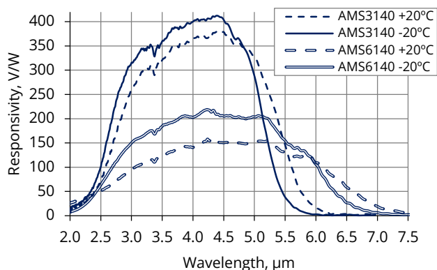
FIGURE 4. Spectral characteristics for different temperatures of detection chip
