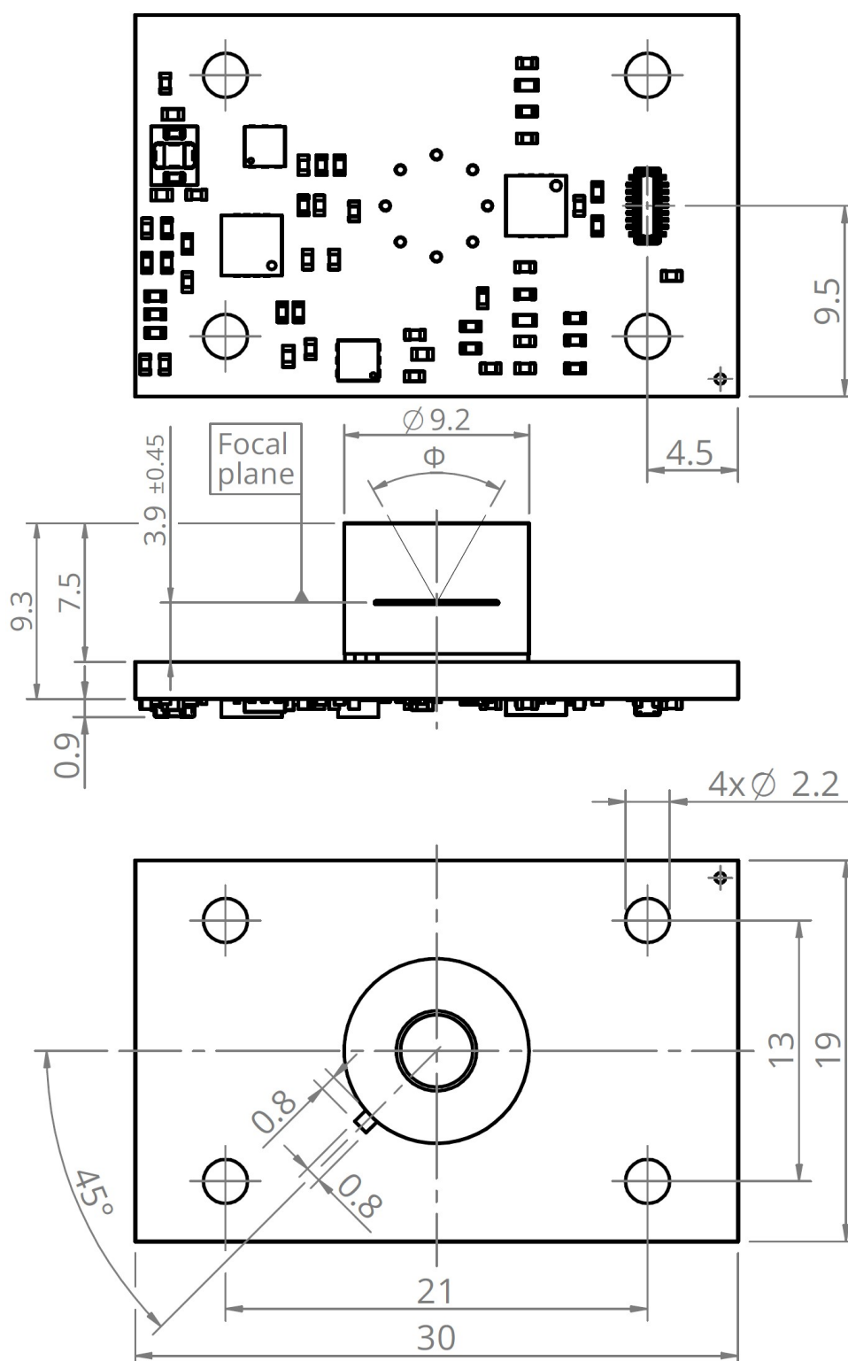
FIGURE 20. Dimensions of AMS3140-01/AMS6140-01 (given in mm)
