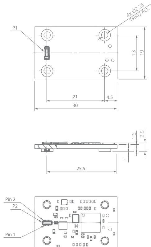
FIGURE 4. Dimensions of the AMS-DIG-PROC (given in mm)
