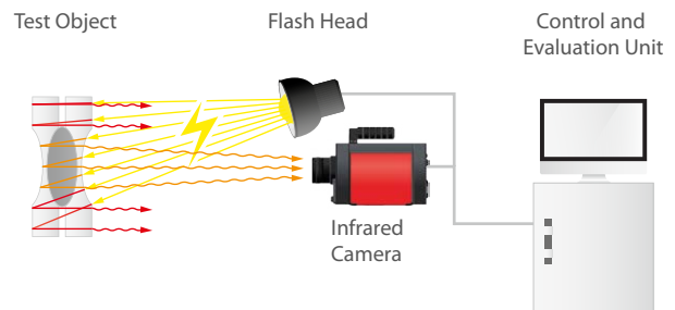
Reflexive order
