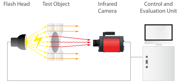
Transmissive order
